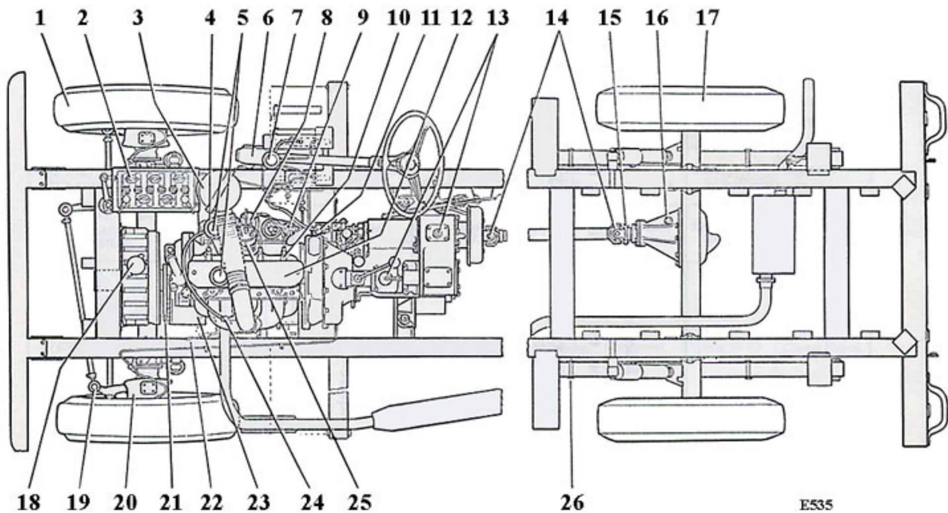
Maintenance diagram, Petrol model illustrated
